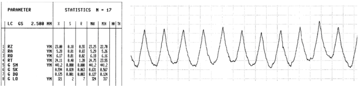
Fig. 4. Results for the same roughness standard obtained from Perthen S8P [10].
