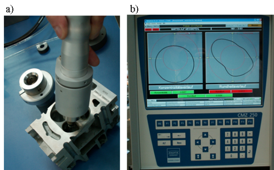
Fig. 1. Example of roundness measurement with a Hommel Etamic probing head (a) and a presentation of the results (b).
