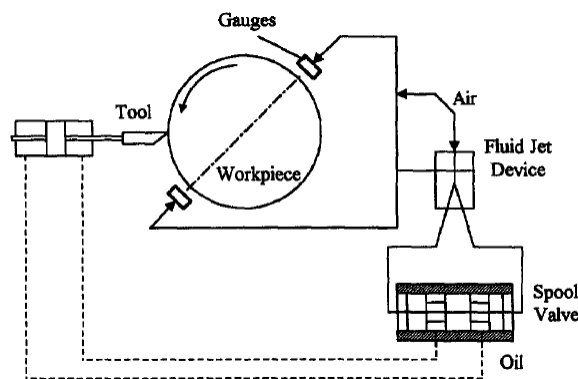
Fig. 14. In-process measurement with hydraulic correction of the cutting tool position [21].
